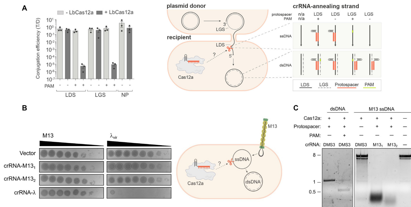
Figure 2. Cas12a does not detectably cis -cleave invasive ssDNA in bacteria. (A) Conjugation efficiency for plasmid cis -targeting in P. aeruginosa PAO1 strain. During conjugation, the donor is nicked and the leading strand (LDS) is transferred as ssDNA to the wildtype (-LbCas12a) or LbCas12a-expressing (+LbCas12a) recipient cell via the mating pilus. LbCas12a was co-expressed with crRNAs complementary to a DMS3 protospacer cloned into the leading (LDS) or lagging (LGS) strand, with (+) or without (-) the correct protospacer adjacent motif (PAM). T/D indicates the ratio of transconjugants to donors. Data are presented as mean \pm SEM ( n = 3 ). LDS, complementary protospacer is on leading strand; LGS, complementary protospacer is on lagging strand; NP, no protospacer on plasmid. (B) Plaque assay for phage cis -targeting in E. coli BW25113 F' strain. Bacterial lawns were infected with dsDNA \lambda_{vir} or with M13, which enters and leaves the cell as ssDNA but replicates via a dsDNA intermediate. LbCas12a was co-expressed in bacteria with crRNA complementary to M13 positive strand (without PAM) or \lambda_{vir} (with PAM) during phage infection. Bacterial clearance (black) indicates phage replication. (C) In vitro LbCas12a cleavage assay on dsDNA template encoding DMS3 protospacer or M13 ssDNA.
