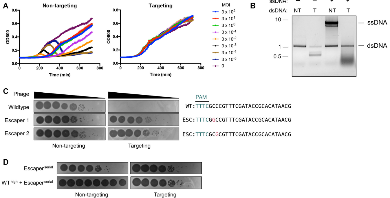
Figure 1. Cas12a targeting does not elicit abortive infection or prevent the rise of phage escapers. (A) Growth curves of P. aeruginosa PAO1 tn7::LbCas12a strain expressing targeting or non-targeting crRNAs infected with \phi DMS3 at multiplicities of infection (MOI) indicated in legend. (B) In vitro LbCas12a cis - and trans -cleavage assay with dsDNA template (plus or minus PAM) and ssDNA. dsDNA template encodes same protospacer encoded in \phi DMS3 for experiments in (A). (C) Phage plaque assays with ten-fold serial dilutions of wildtype or mutated \phi JBD30 phage. Bacterial clearance (black) indicates phage replication. Sequences of the targeted phage gene show mutated nucleotides (magenta) in phages able to escape Cas12a targeting. (D) Phage plaque assays in which targeting and non-targeting strains were infected with ten-fold serial dilutions of escaper phage alone or with escaper phage and a high titer of targeted wildtype phage. PAM, protospacer adjacent motif (teal); WT, wildtype phage; ESC, escaper phage. NT, non-target due to lack of PAM; T, target with PAM.
